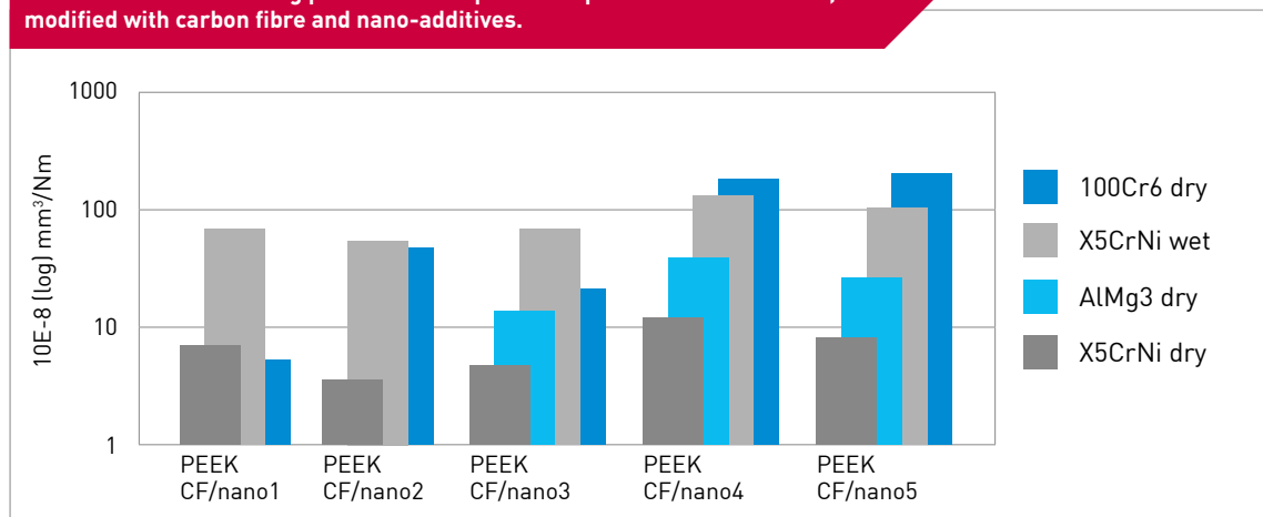
Wear of tribologically modified LUVOCOM® under dry running conditions / with grease and various counteracting partners. Example of compounds based on PEEK, modified with carbon fibre and nano-additives.
